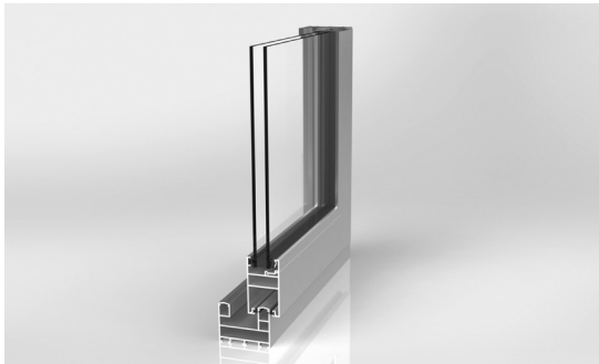
Profil Non-insulated aluminium sliding system.
