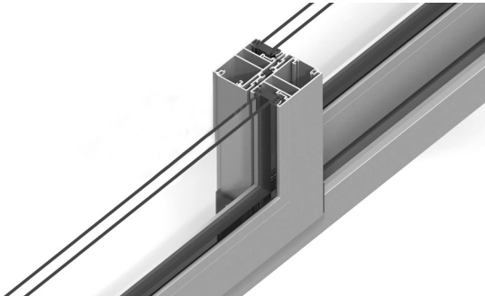
Vertical frame Increased water- and windtightness by three sealing levels within the labyrinth area.
